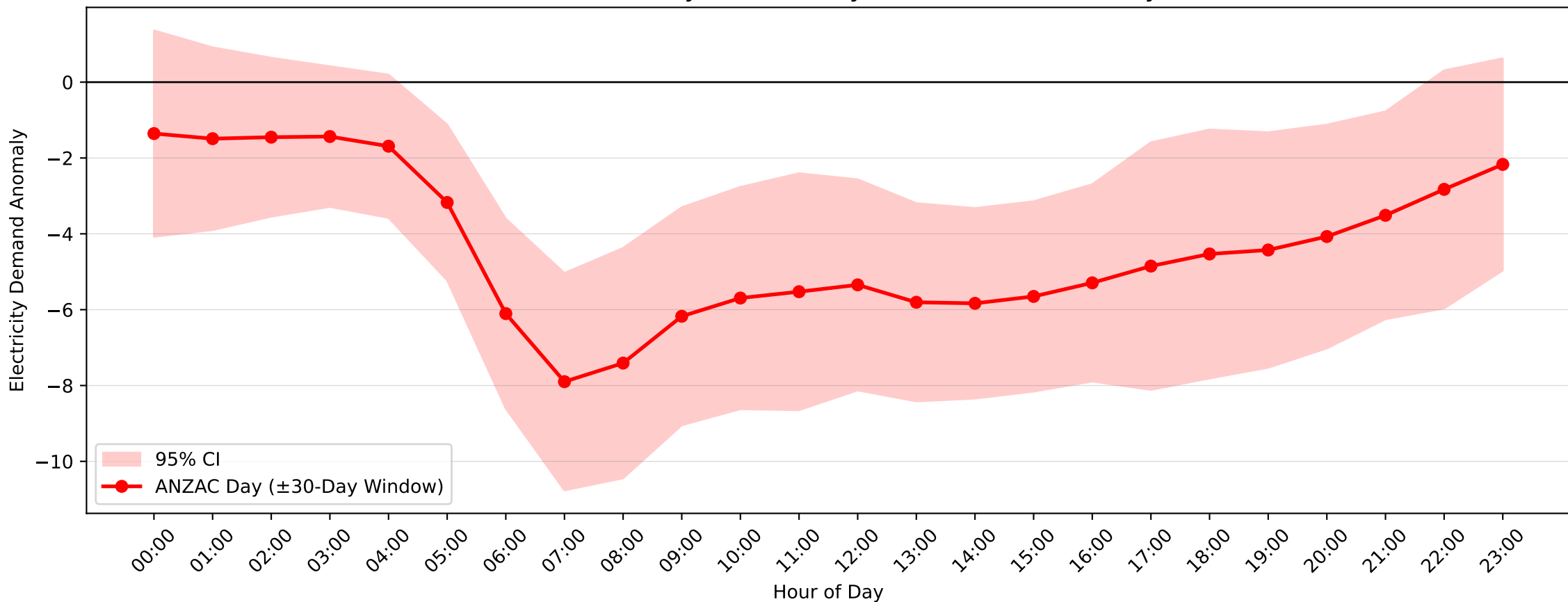
Sefton Demand Anomaly: ANZAC Day (2004-2017, \pm 30 -Day Window)
